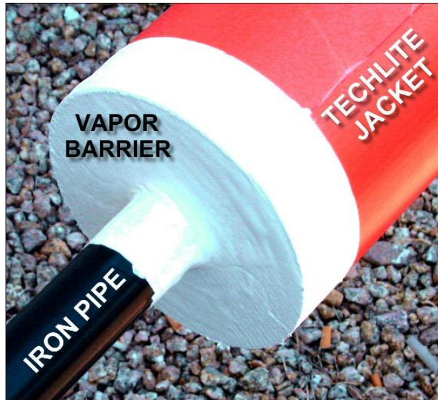
Photo 3: Special fittings
