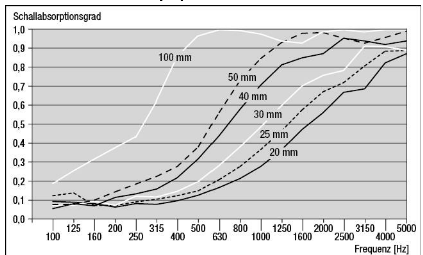
Diagram 2: Degree of sound absorption of Basotect® B / B EcoBalanced as a function of the thickness, according to ISO 10534-2 (impedance tube).
