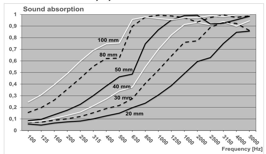
Diagram 2: Degree of sound absorption of Basotect® Dark EcoBalanced as a function of the thickness, according to ISO 10534-2 (impedance tube).
