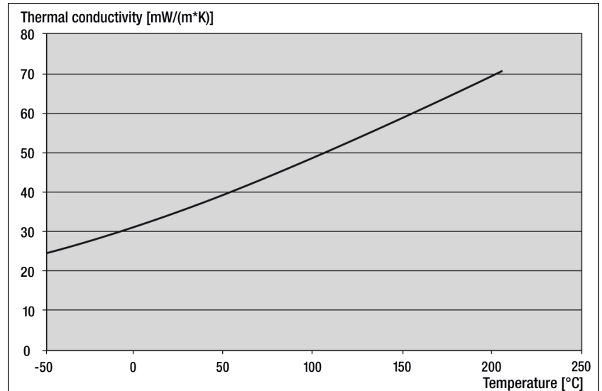
Diagram 2: Thermal conductivity of Basotect® G+ / G+ EcoBalanced.
