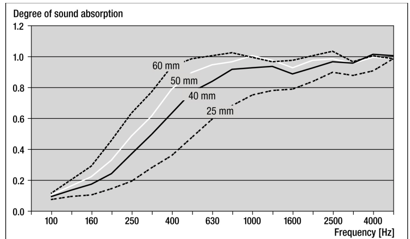
Diagram 4: Degree of sound absorption of Basotect® G+ / G+ EcoBalanced as a function of the thickness, according to DIN EN ISO 354 (reverberation room)
