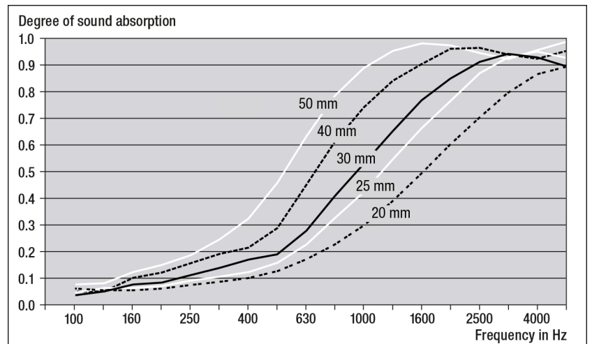
Diagram 3: Degree of sound absorption of Basotect® G+ / G+ EcoBalanced as a function of the thickness, according to DIN EN ISO 10534-2 (impedance tube).
